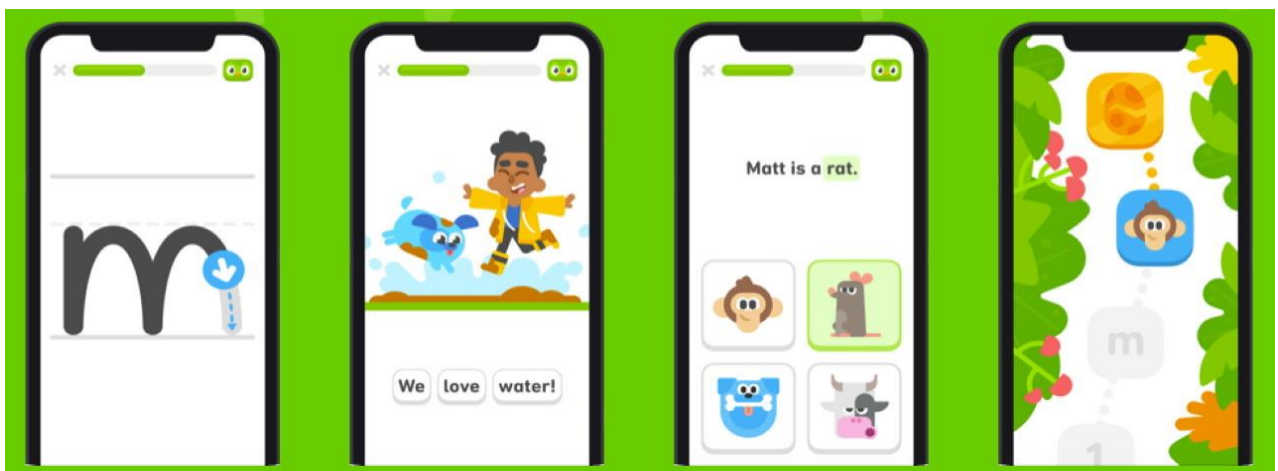
Slika 7. (Izvor: https://apps.apple.com/us/app/duolingo-abc-learn-to-read/id1440502568 )
