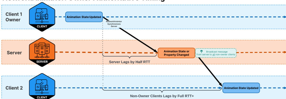
Slika 57 - Client Authoritative [22]
