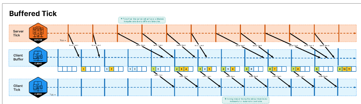
Slika 55 - Buffered tick [21]
