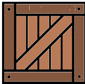
Slika 16. LootBox (Logomakr,2023)
