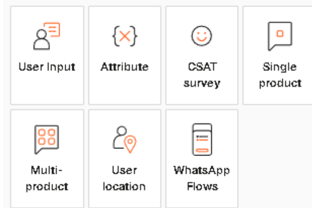
Slika 7.- Chatbot receives
